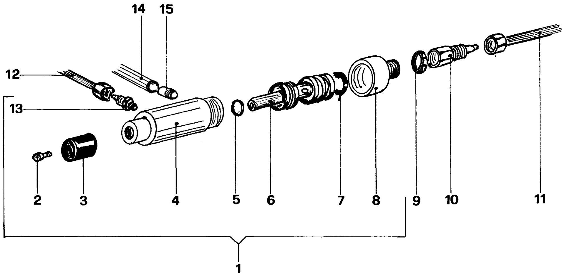
Water feed selector valve
