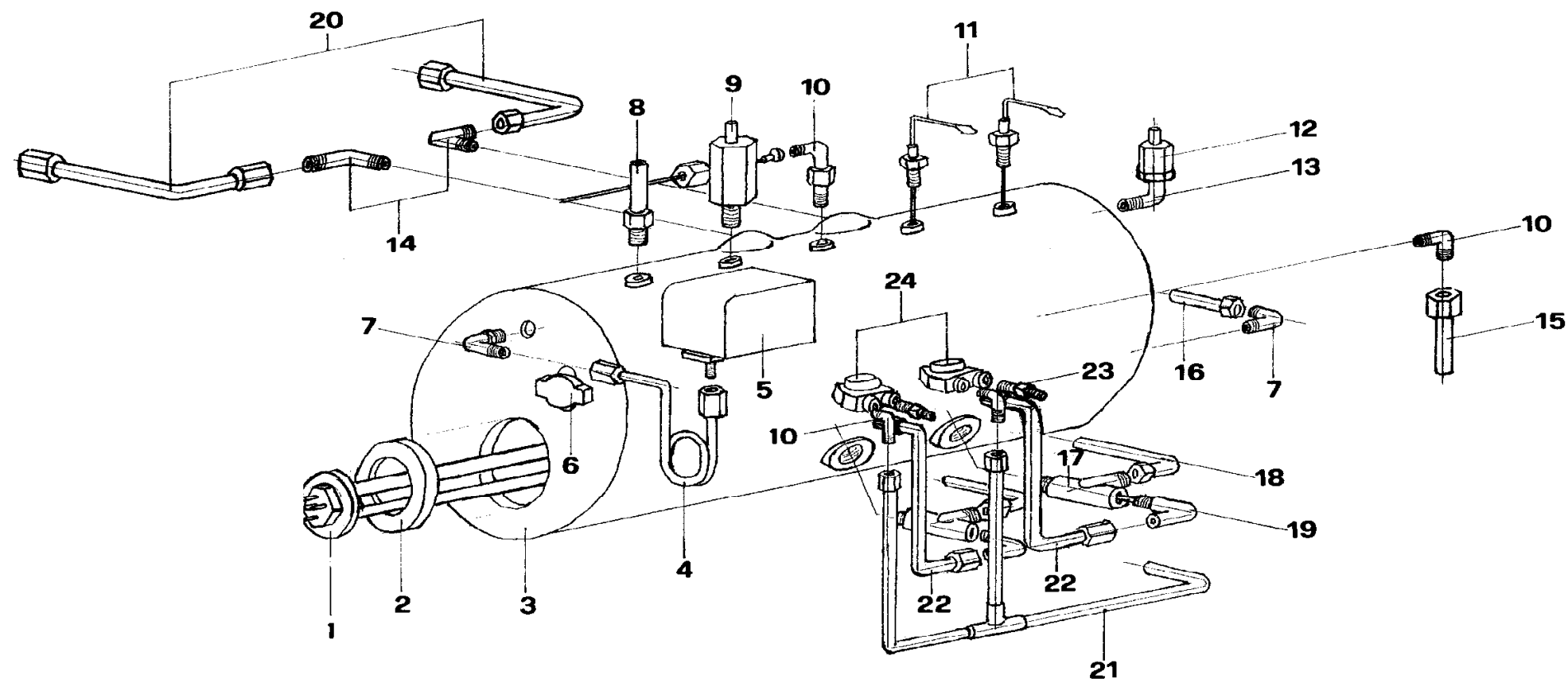
Boiler / hydraulic parts - Raffaello A 2 groups
