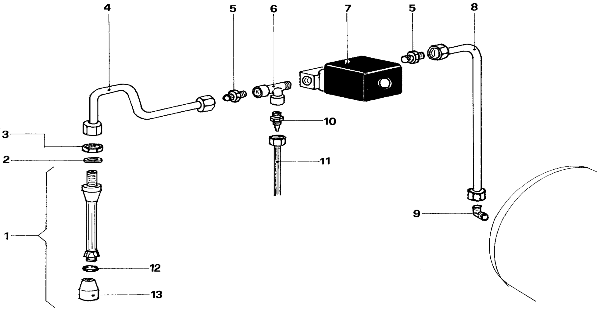
Hot water valve
