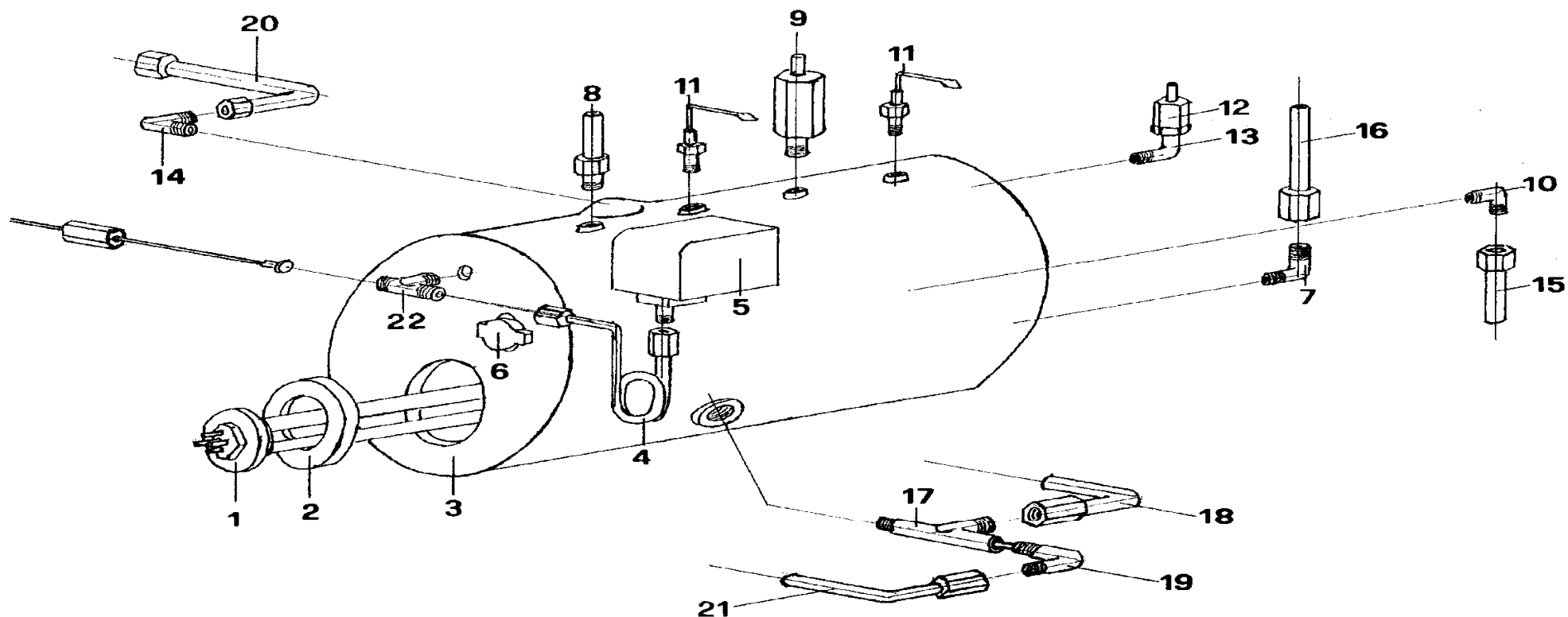
Boiler / hydraulic parts - Raffaello S 1 group
