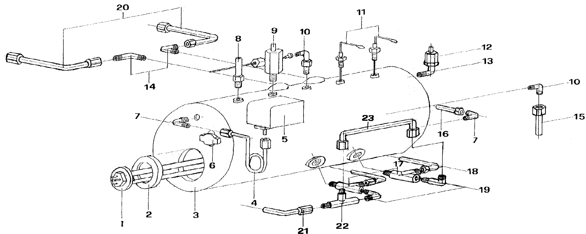
Boiler / hydraulic parts - Raffaello A 1 group
