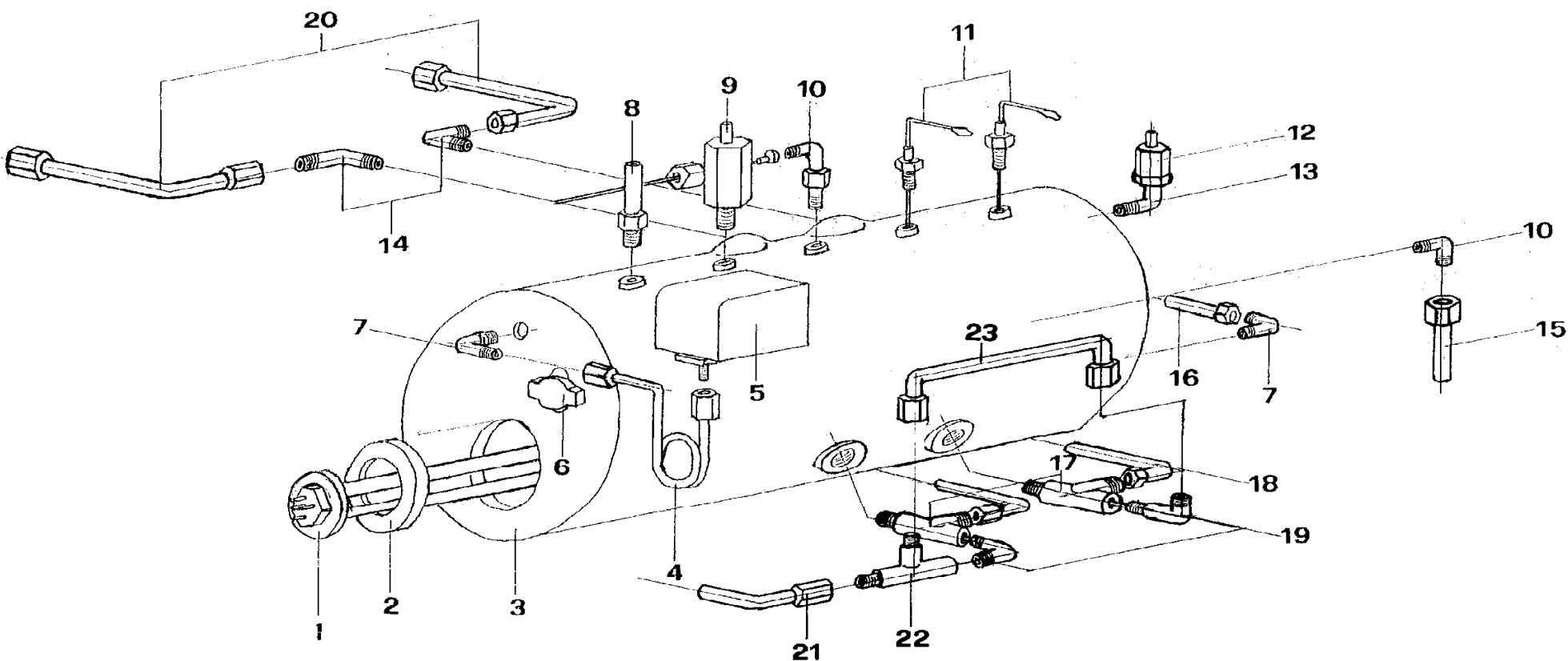
Boiler / hydraulic parts - Raffaello S 2 groups
